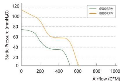
Air Performance
