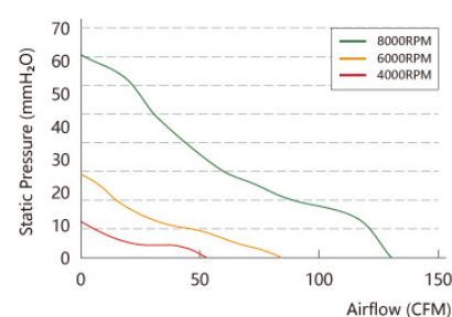
Air Performance
