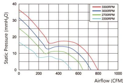
Air Performance
